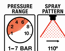
TTI TWIN JET AIR INDUCTION TWIN FLAT FAN SPRAY TIP
